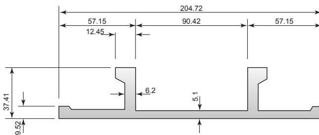
Cross Section of Standard Vertical Rail Dimensions Millimeter (mm)
