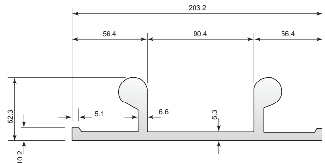
Cross Section of Heavy-Duty Vertical Rail Dimensions Millimeter (mm)
